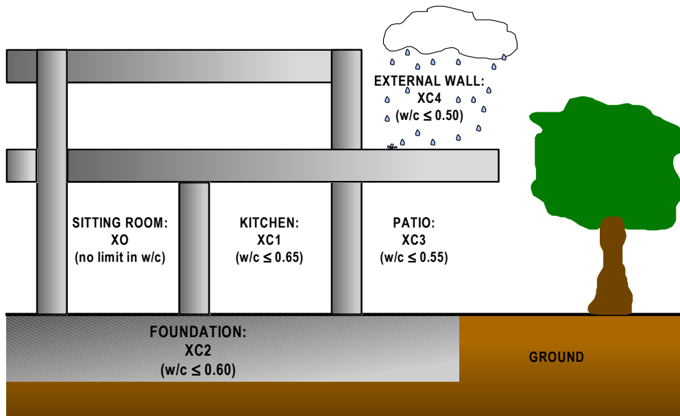
Figure 1 Example of different concrete mixtures which should be adopted in small house according to EN 206.
