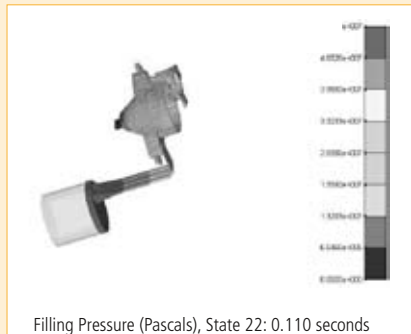
Filling Pressure (Pascals), State 22: 0.110 seconds
